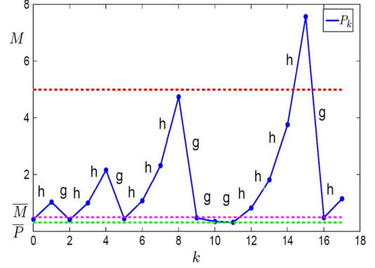
Fig. 2. Packet arrival sequence.
